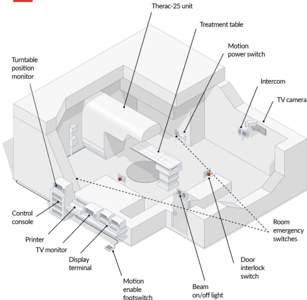
Therac-25 séma, Source: createdigital.org.au / Diagram adapted from Leveson (1995)
